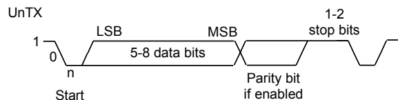
Figure 19-2. UART Character Frame
