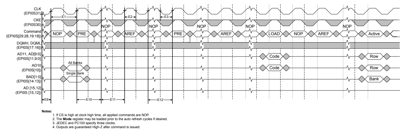
Figure 32-18. SDRAM Initialization and Load Mode Register Timing
